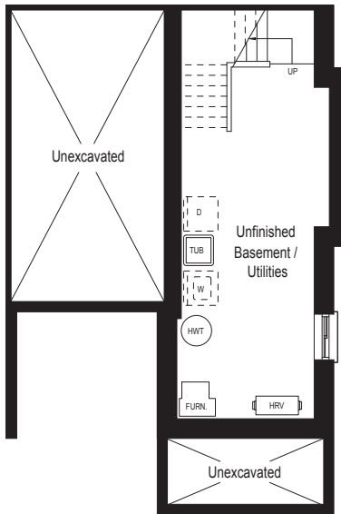
BASEMENT FLOOR PLAN
