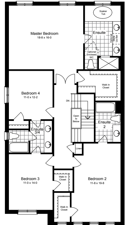
Second Floor Plan Elevation C
