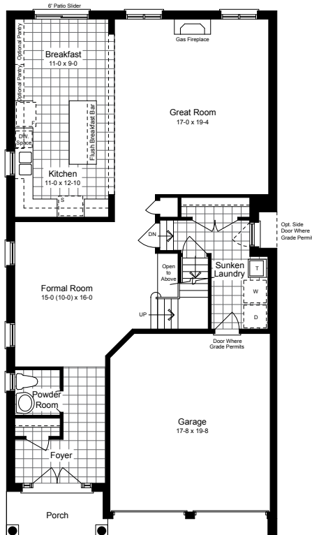
Ground Floor Plan Elevation C
