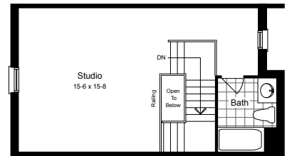
Optional Loft Plan Elevation A, B and C
